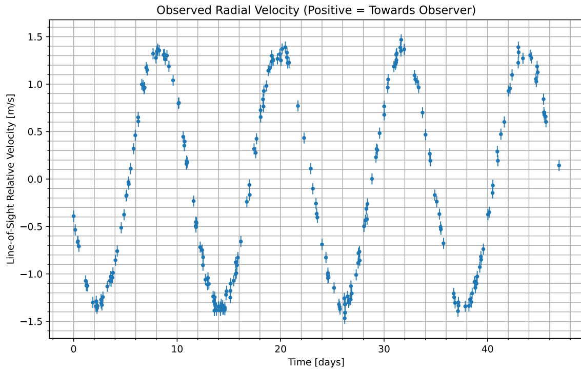
Figure 1: We have isolated the radial velocity of the host star due to the candidate planet. Data begins at UTC 2078-11-12/08:08. Positive values indicate the velocity at which the star is moving towards us; negative indicate the velocity at which it is moving away.
