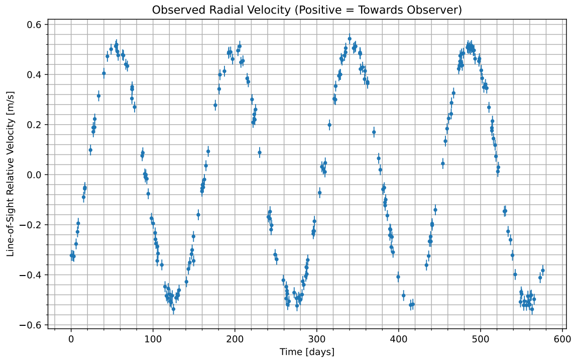
Figure 1: We have isolated the radial velocity of the host star due to the candidate planet. Data begins at UTC 2090-03-20/01:46. Positive values indicate the velocity at which the star is moving towards us; negative indicate the velocity at which it is moving away.
