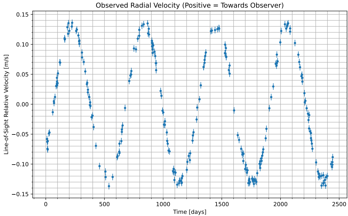
Figure 1: We have isolated the radial velocity of the host star due to the candidate planet. Data begins at UTC 2083-05-10/04:13. Positive values indicate the velocity at which the star is moving towards us; negative indicate the velocity at which it is moving away.
