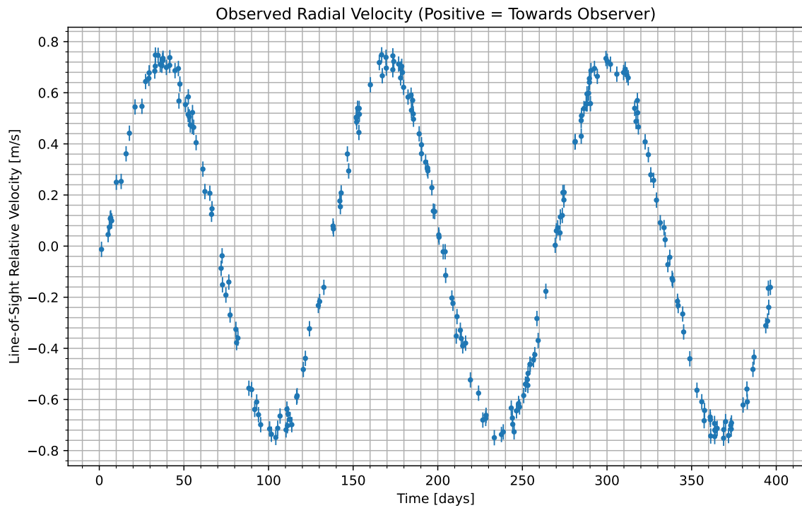
Figure 1: We have isolated the radial velocity of the host star due to the candidate planet. Data begins at UTC 2077-02-04/23:47. Positive values indicate the velocity at which the star is moving towards us; negative indicate the velocity at which it is moving away.
