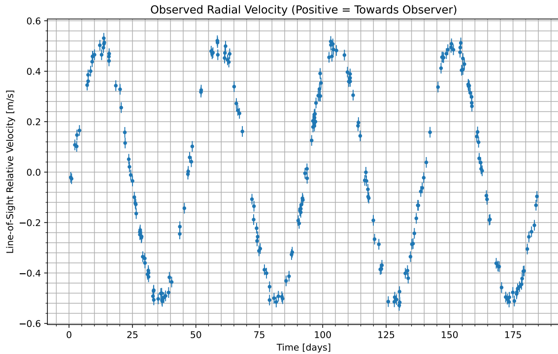
Figure 1: We have isolated the radial velocity of the host star due to the candidate planet. Data begins at UTC 2100-03-11/22:36. Positive values indicate the velocity at which the star is moving towards us; negative indicate the velocity at which it is moving away.
