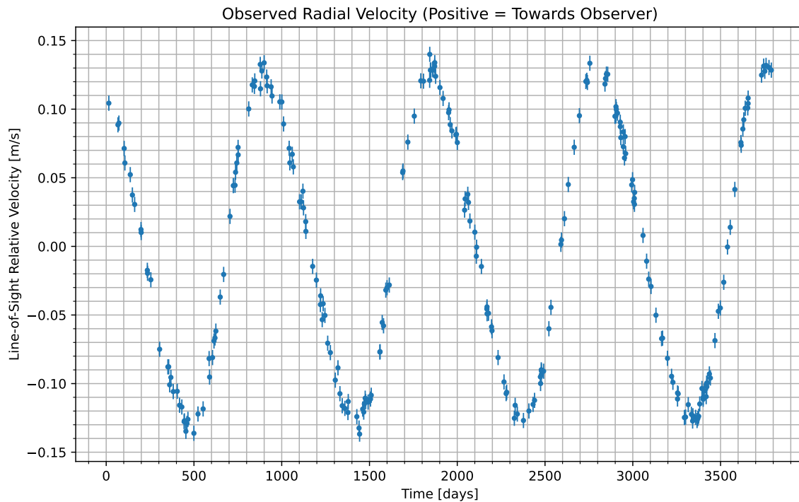
Figure 1: We have isolated the radial velocity of the host star due to the candidate planet. Data begins at UTC 2086-10-12/13:17. Positive values indicate the velocity at which the star is moving towards us; negative indicate the velocity at which it is moving away.
