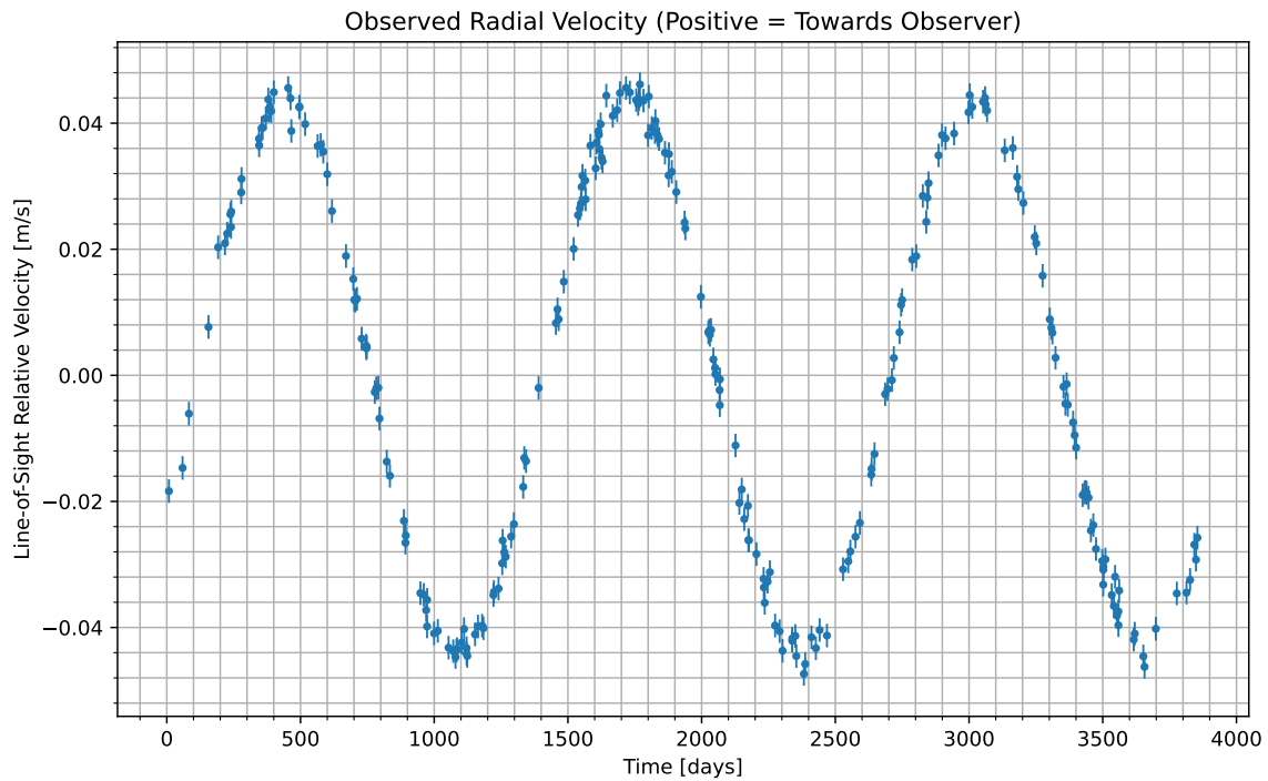
Figure 1: We have isolated the radial velocity of the host star due to the candidate planet. Data begins at UTC 2082-10-19/02:09. Positive values indicate the velocity at which the star is moving towards us; negative indicate the velocity at which it is moving away.
