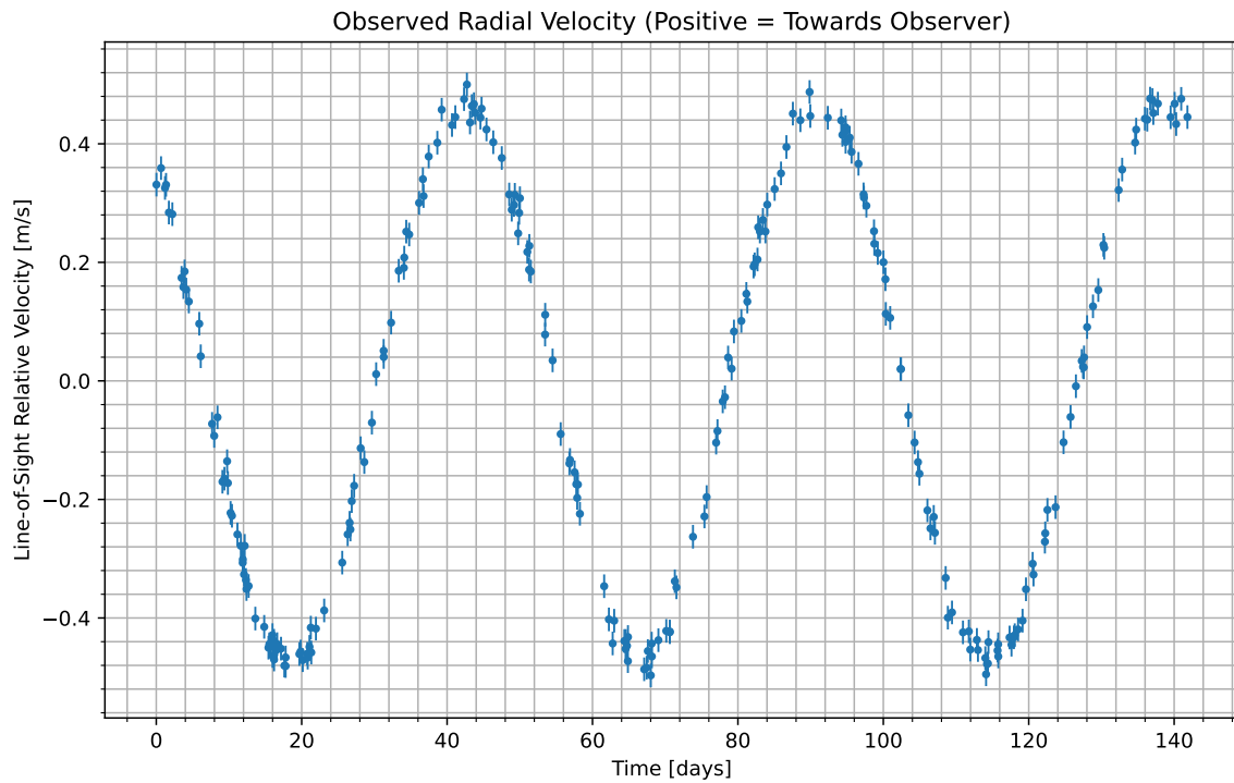
Figure 1: We have isolated the radial velocity of the host star due to the candidate planet. Data begins at UTC 2080-06-29/02:49. Positive values indicate the velocity at which the star is moving towards us; negative indicate the velocity at which it is moving away.
