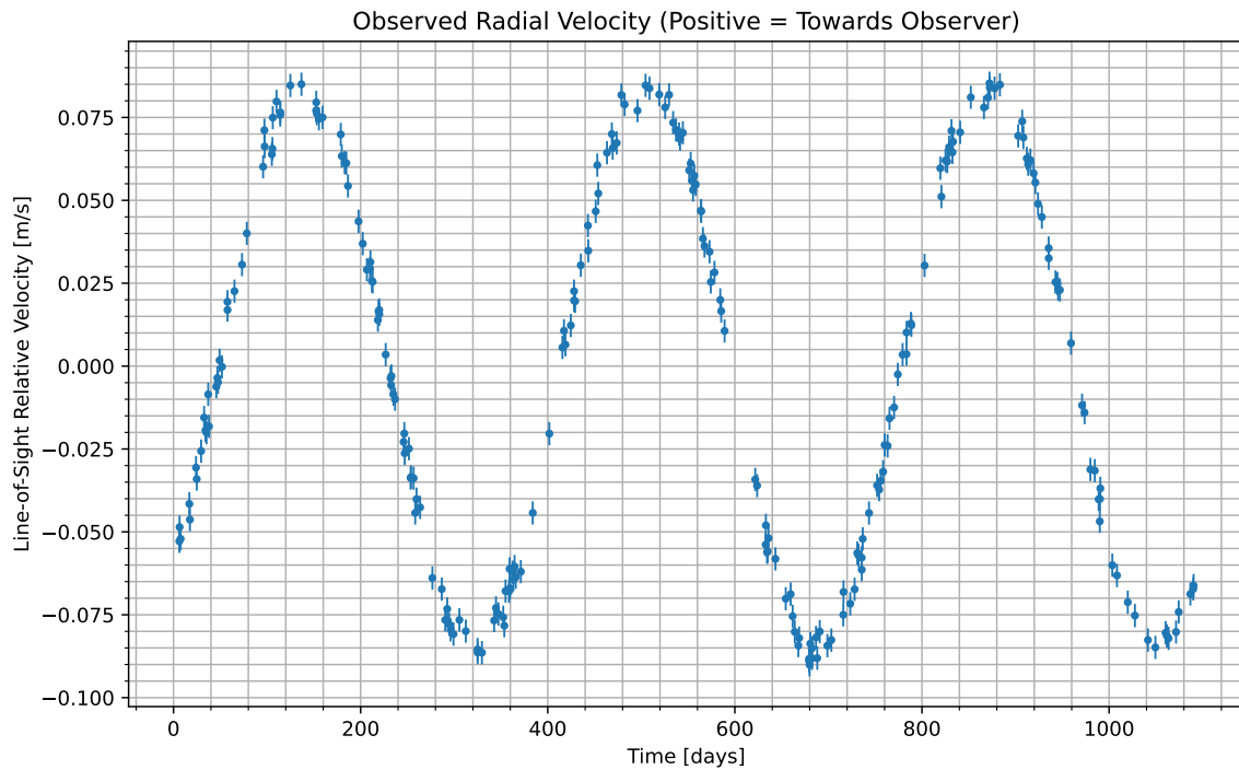
Figure 1: We have isolated the radial velocity of the host star due to the candidate planet. Data begins at UTC 2086-01-29/14:23. Positive values indicate the velocity at which the star is moving towards us; negative indicate the velocity at which it is moving away.
