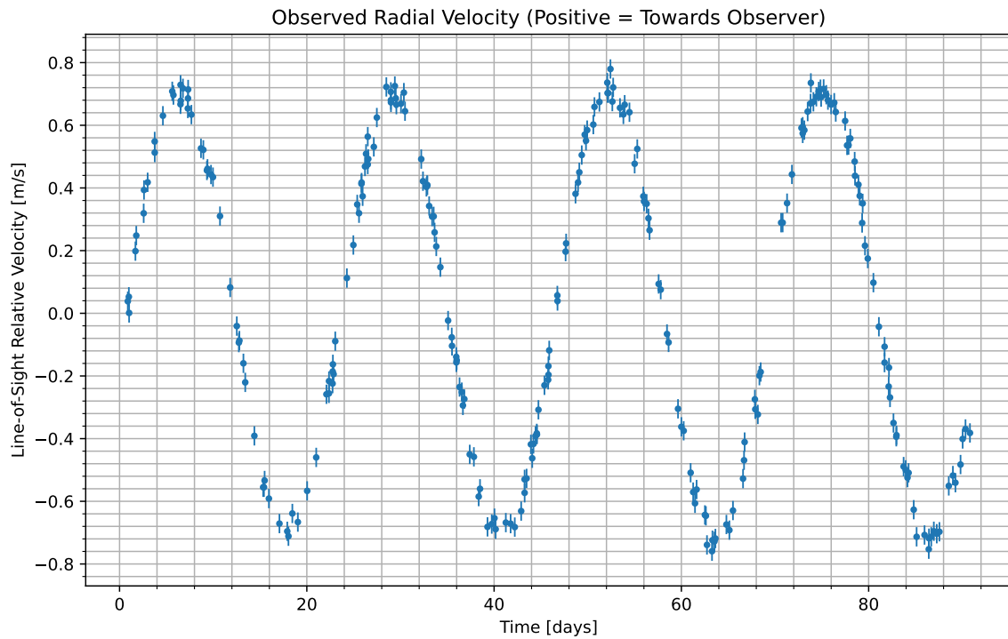
Figure 1: We have isolated the radial velocity of the host star due to the candidate planet. Data begins at UTC 2082-06-22/02:18. Positive values indicate the velocity at which the star is moving towards us; negative indicate the velocity at which it is moving away.
