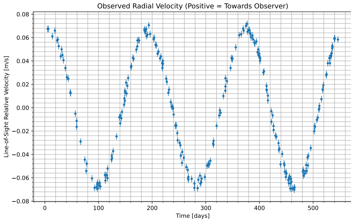
Figure 1: We have isolated the radial velocity of the host star due to the candidate planet. Data begins at UTC 2068-12-20/16:23. Positive values indicate the velocity at which the star is moving towards us; negative indicate the velocity at which it is moving away.
