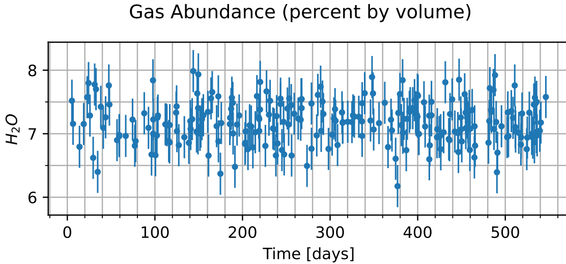
Figure 3: Concentration of various additional gases in the atmosphere of the candidate planet versus time. Note that the y-axis will usually only show the variation multiplied by some factor, shown in the upper left, and then added to some normal amount, also in the upper-left.
