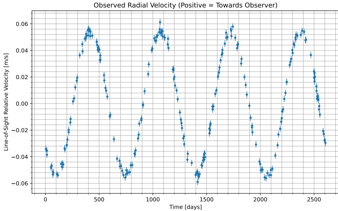
Figure 1: We have isolated the radial velocity of the host star due to the candidate planet. Data begins at UTC 2073-09-19/20:11. Positive values indicate the velocity at which the star is moving towards us; negative indicate the velocity at which it is moving away.
