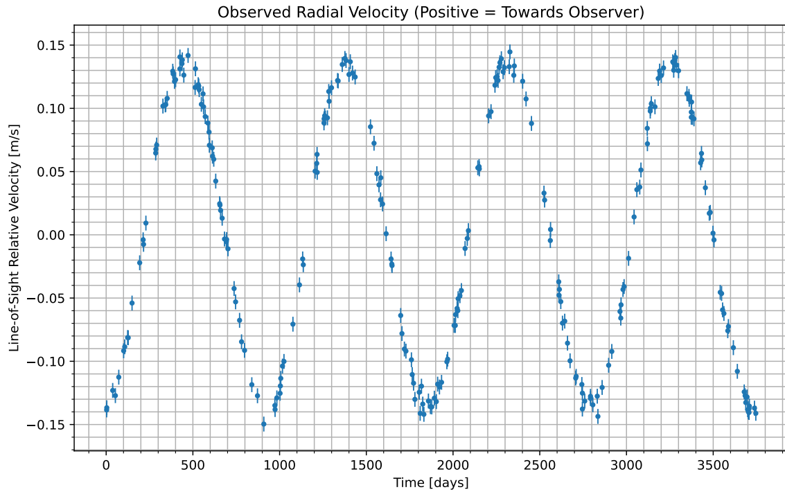
Figure 1: We have isolated the radial velocity of the host star due to the candidate planet. Data begins at UTC 2088-10-31/17:27. Positive values indicate the velocity at which the star is moving towards us; negative indicate the velocity at which it is moving away.
