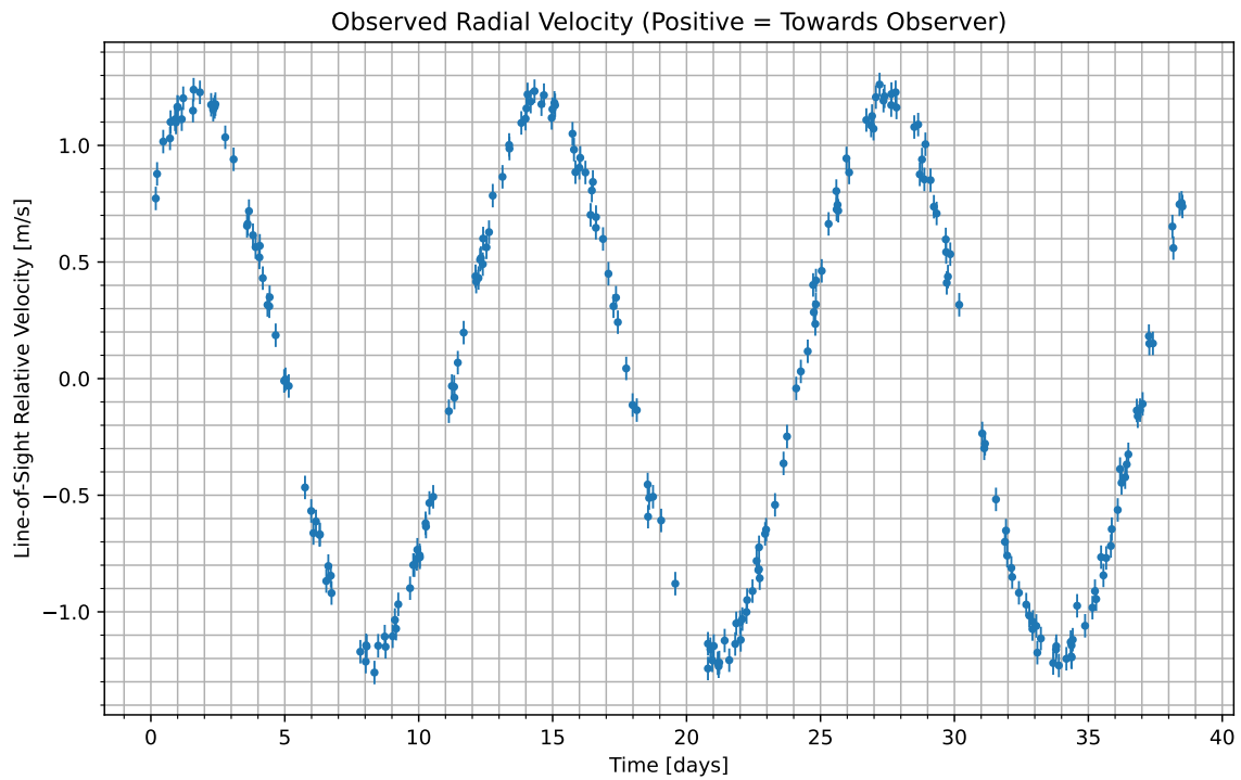
Figure 1: We have isolated the radial velocity of the host star due to the candidate planet. Data begins at UTC 2087-01-17/12:07. Positive values indicate the velocity at which the star is moving towards us; negative indicate the velocity at which it is moving away.
