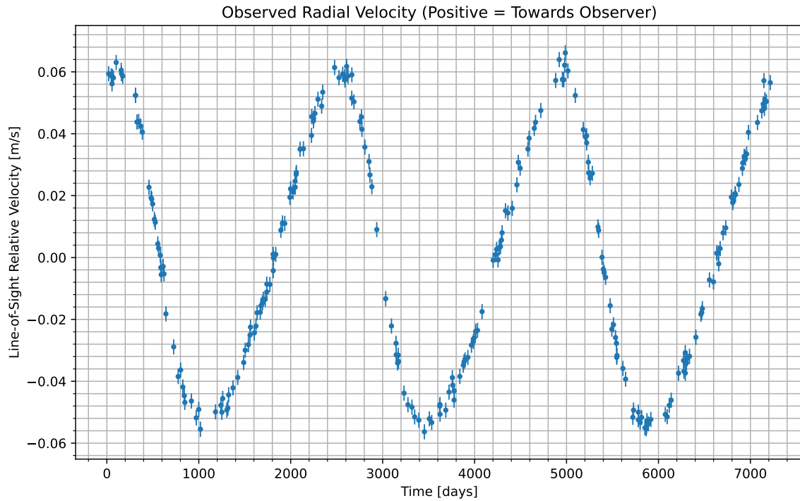
Figure 1: We have isolated the radial velocity of the host star due to the candidate planet. Data begins at UTC 2065-03-07/11:29. Positive values indicate the velocity at which the star is moving towards us; negative indicate the velocity at which it is moving away.
