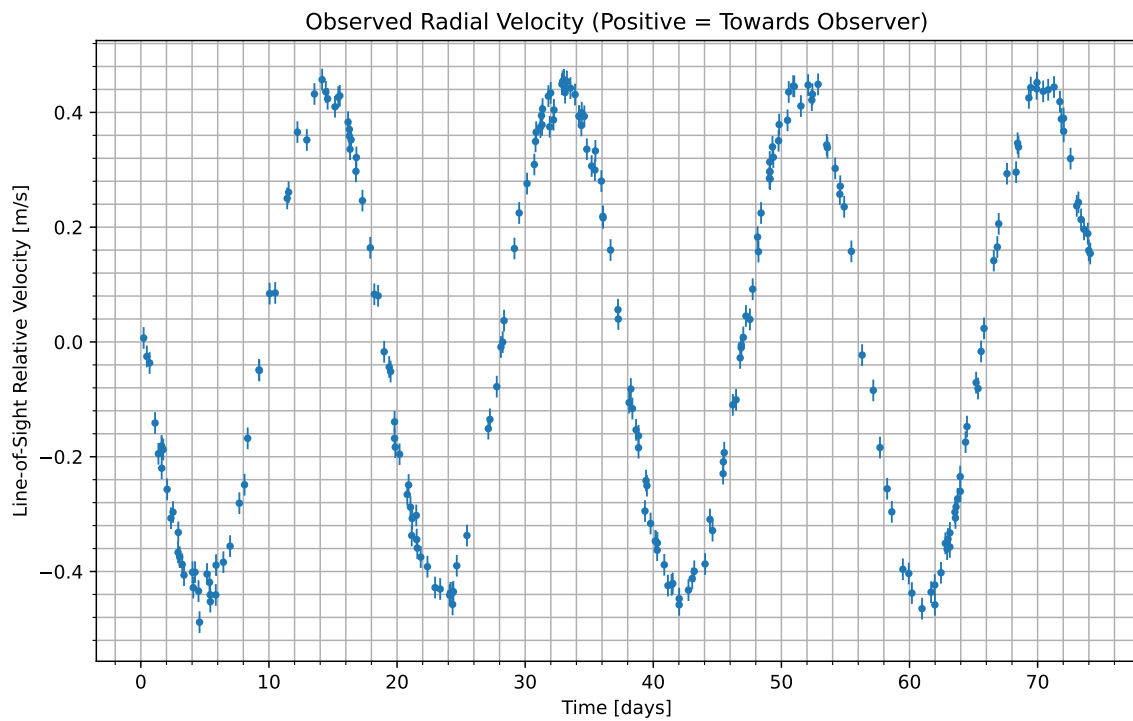
Figure 1: We have isolated the radial velocity of the host star due to the candidate planet. Data begins at UTC 2093-06-06/21:39. Positive values indicate the velocity at which the star is moving towards us; negative indicate the velocity at which it is moving away.
