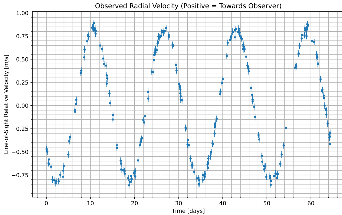
Figure 1: We have isolated the radial velocity of the host star due to the candidate planet. Data begins at UTC 2091-07-24/23:37. Positive values indicate the velocity at which the star is moving towards us; negative indicate the velocity at which it is moving away.
