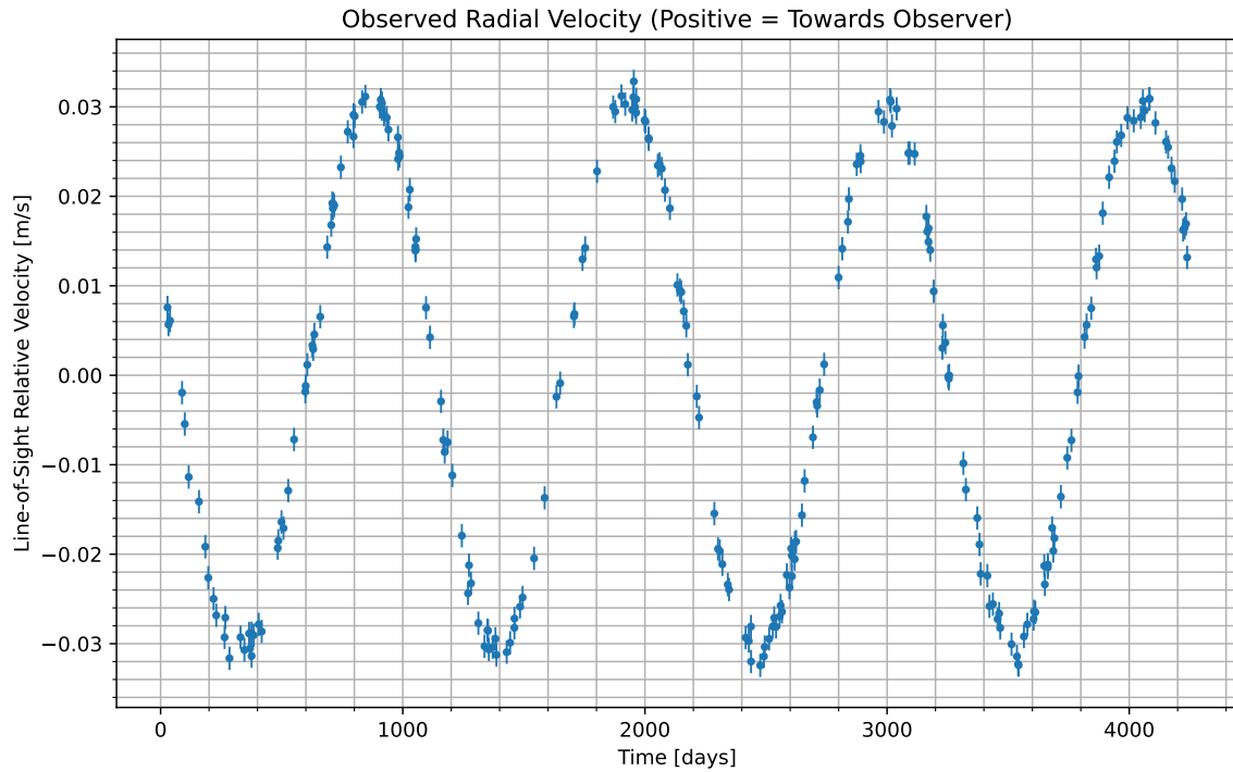
Figure 1: We have isolated the radial velocity of the host star due to the candidate planet. Data begins at UTC 2078-05-17/23:18. Positive values indicate the velocity at which the star is moving towards us; negative indicate the velocity at which it is moving away.
