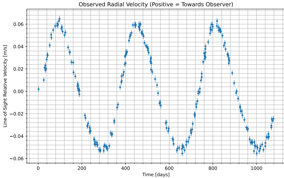
Figure 1: We have isolated the radial velocity of the host star due to the candidate planet. Data begins at UTC 2069-09-02/23:09. Positive values indicate the velocity at which the star is moving towards us; negative indicate the velocity at which it is moving away.
