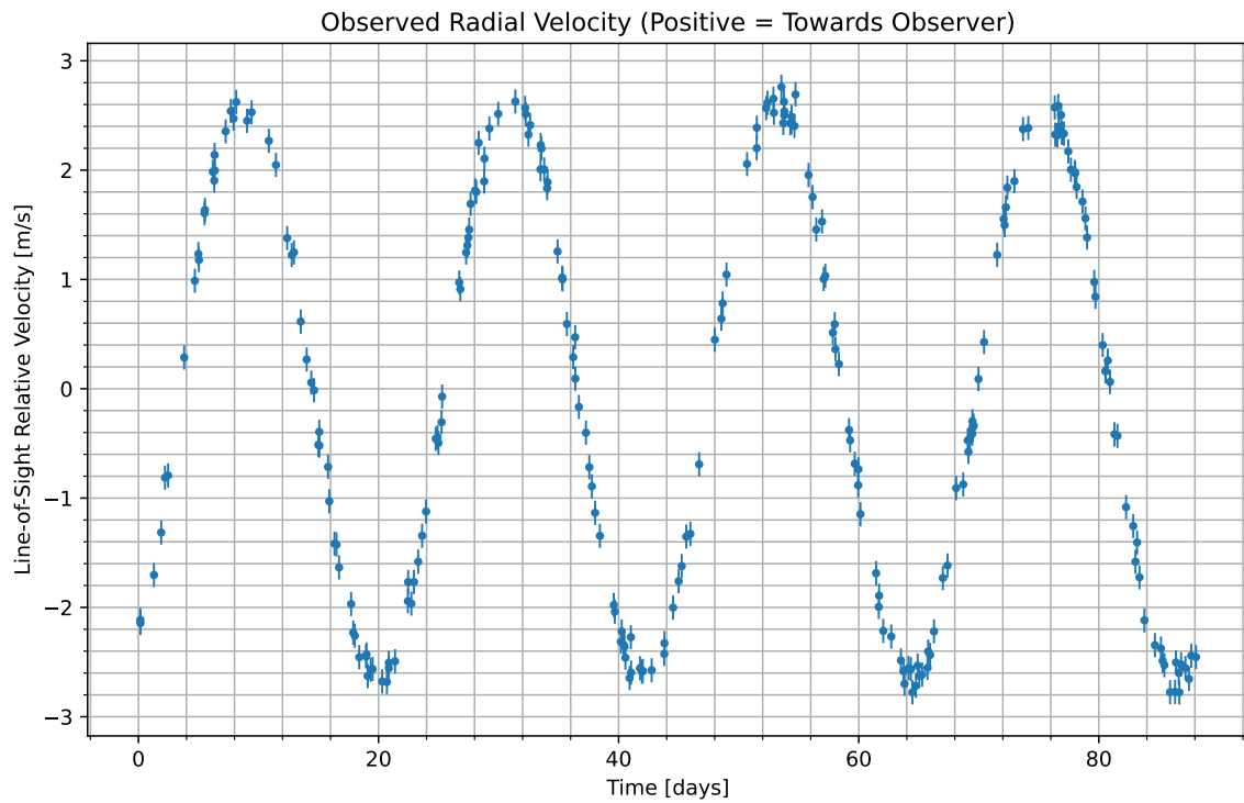
Figure 1: We have isolated the radial velocity of the host star due to the candidate planet. Data begins at UTC 2091-06-25/10:21. Positive values indicate the velocity at which the star is moving towards us; negative indicate the velocity at which it is moving away.
