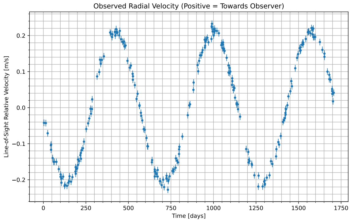
Figure 1: We have isolated the radial velocity of the host star due to the candidate planet. Data begins at UTC 2077-05-15/00:25. Positive values indicate the velocity at which the star is moving towards us; negative indicate the velocity at which it is moving away.
