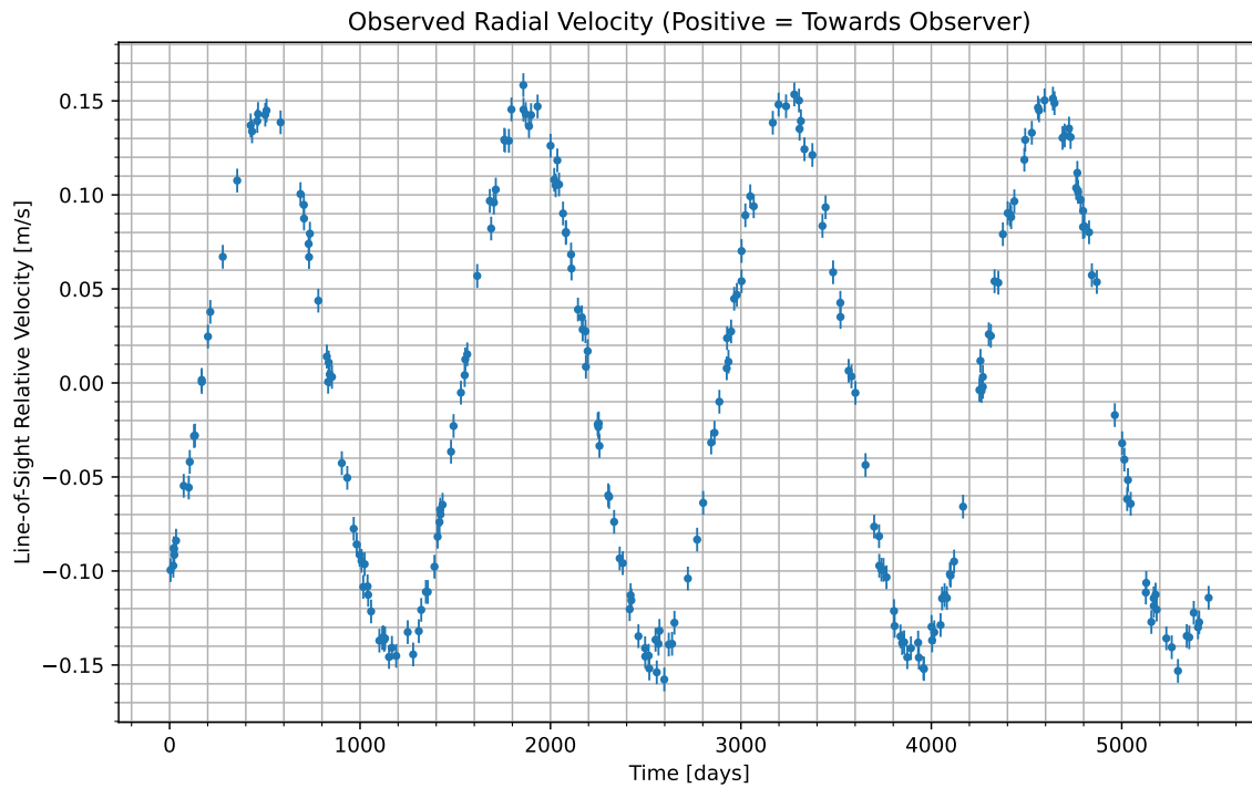
Figure 1: We have isolated the radial velocity of the host star due to the candidate planet. Data begins at UTC 2078-06-24/14:21. Positive values indicate the velocity at which the star is moving towards us; negative indicate the velocity at which it is moving away.
