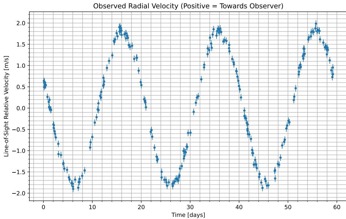
Figure 1: We have isolated the radial velocity of the host star due to the candidate planet. Data begins at UTC 2098-06-08/13:53. Positive values indicate the velocity at which the star is moving towards us; negative indicate the velocity at which it is moving away.
