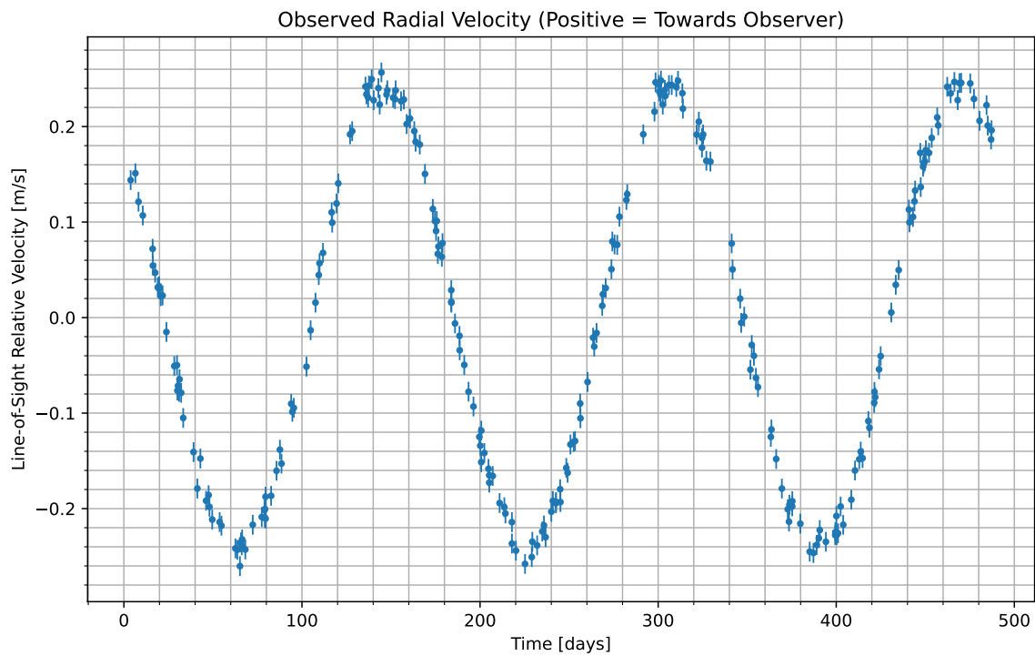
Figure 1: We have isolated the radial velocity of the host star due to the candidate planet. Data begins at UTC 2093-02-23/18:38. Positive values indicate the velocity at which the star is moving towards us; negative indicate the velocity at which it is moving away.
