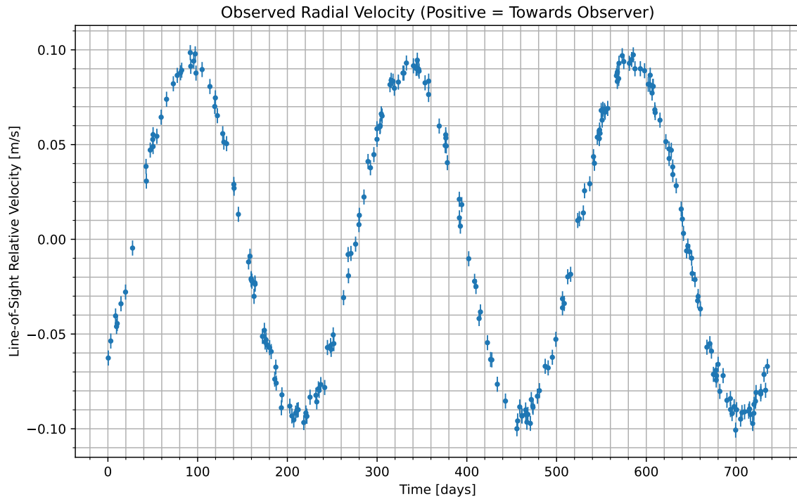
Figure 1: We have isolated the radial velocity of the host star due to the candidate planet. Data begins at UTC 2094-04-27/13:40. Positive values indicate the velocity at which the star is moving towards us; negative indicate the velocity at which it is moving away.
