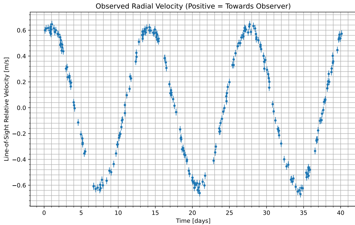
Figure 1: We have isolated the radial velocity of the host star due to the candidate planet. Data begins at UTC 2071-04-29/21:12. Positive values indicate the velocity at which the star is moving towards us; negative indicate the velocity at which it is moving away.
