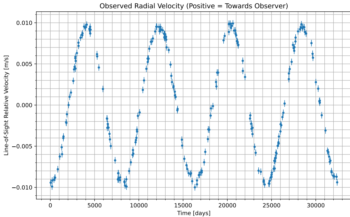
Figure 1: We have isolated the radial velocity of the host star due to the candidate planet. Data begins at UTC 1982-09-10/12:09. Positive values indicate the velocity at which the star is moving towards us; negative indicate the velocity at which it is moving away.
