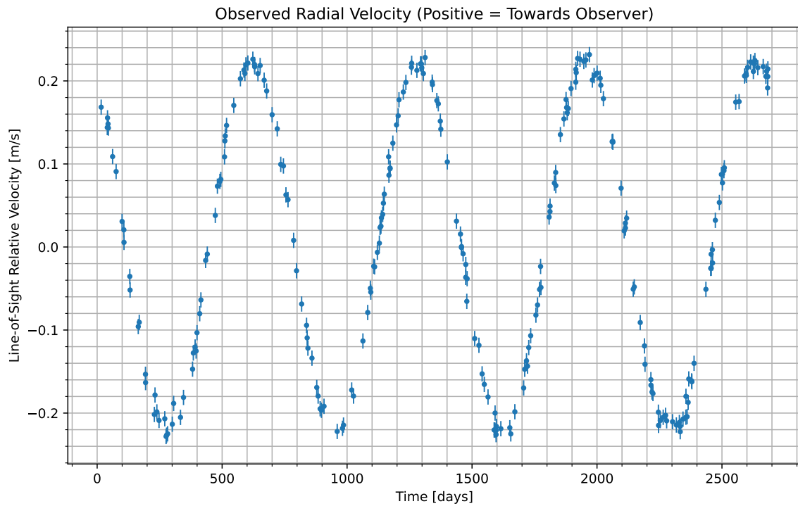
Figure 1: We have isolated the radial velocity of the host star due to the candidate planet. Data begins at UTC 2071-11-27/22:53. Positive values indicate the velocity at which the star is moving towards us; negative indicate the velocity at which it is moving away.
