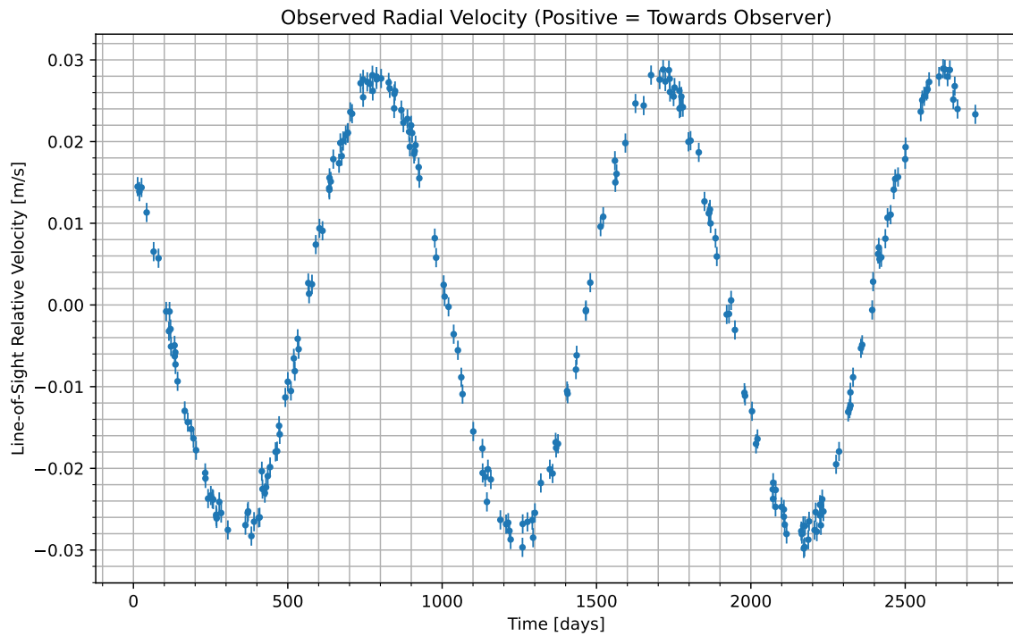
Figure 1: We have isolated the radial velocity of the host star due to the candidate planet. Data begins at UTC 2069-05-14/16:04. Positive values indicate the velocity at which the star is moving towards us; negative indicate the velocity at which it is moving away.
