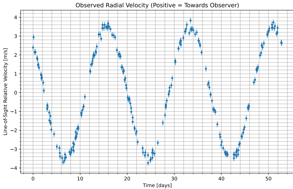
Figure 1: We have isolated the radial velocity of the host star due to the candidate planet. Data begins at UTC 2082-07-12/04:33. Positive values indicate the velocity at which the star is moving towards us; negative indicate the velocity at which it is moving away.
