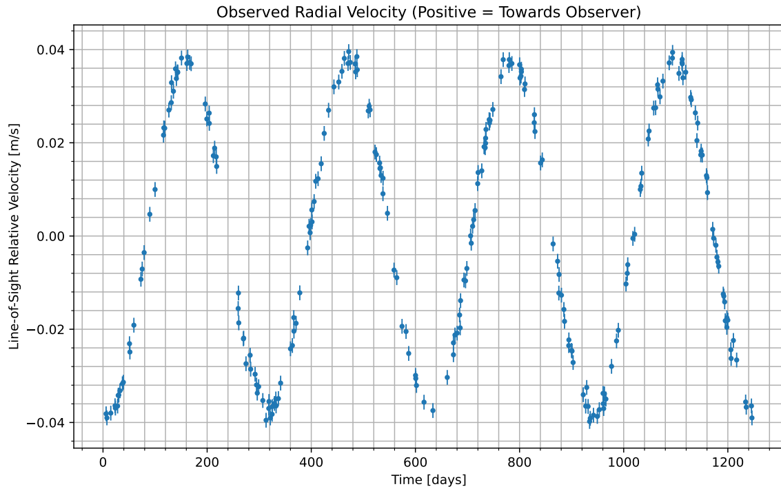
Figure 1: We have isolated the radial velocity of the host star due to the candidate planet. Data begins at UTC 2090-04-04/16:41. Positive values indicate the velocity at which the star is moving towards us; negative indicate the velocity at which it is moving away.
