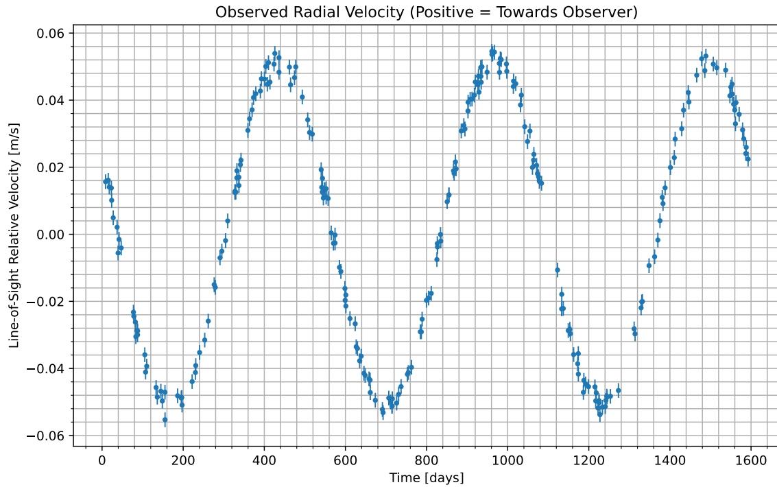
Figure 1: We have isolated the radial velocity of the host star due to the candidate planet. Data begins at UTC 2082-02-20/20:31. Positive values indicate the velocity at which the star is moving towards us; negative indicate the velocity at which it is moving away.
