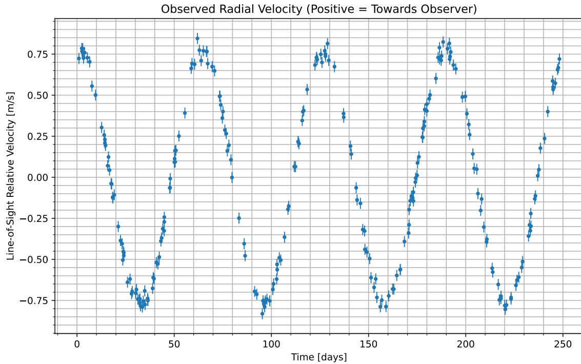
Figure 1: We have isolated the radial velocity of the host star due to the candidate planet. Data begins at UTC 2095-11-21/02:58. Positive values indicate the velocity at which the star is moving towards us; negative indicate the velocity at which it is moving away.
