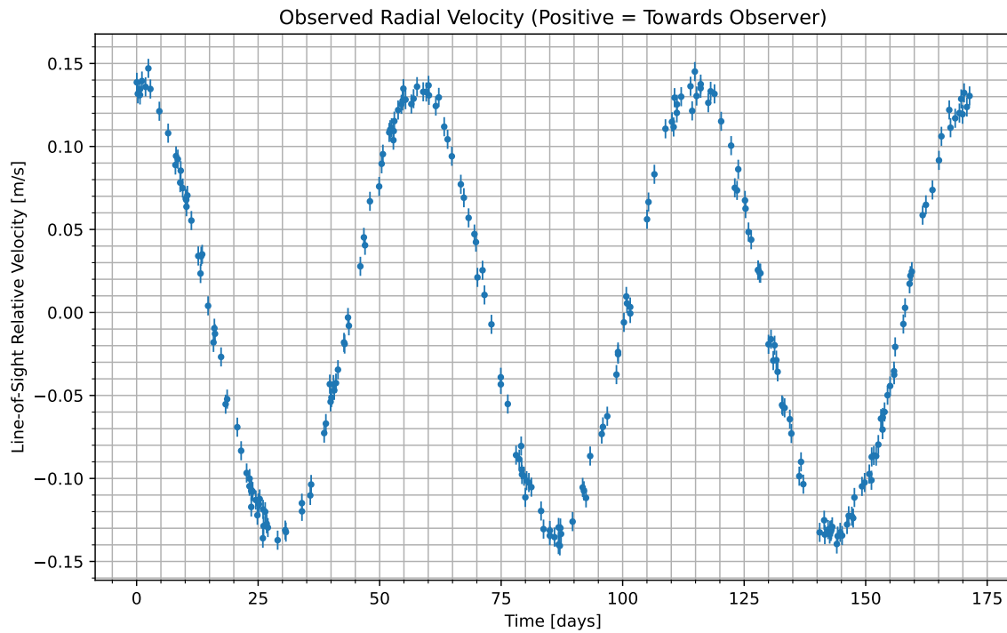
Figure 1: We have isolated the radial velocity of the host star due to the candidate planet. Data begins at UTC 2073-05-17/09:52. Positive values indicate the velocity at which the star is moving towards us; negative indicate the velocity at which it is moving away.
