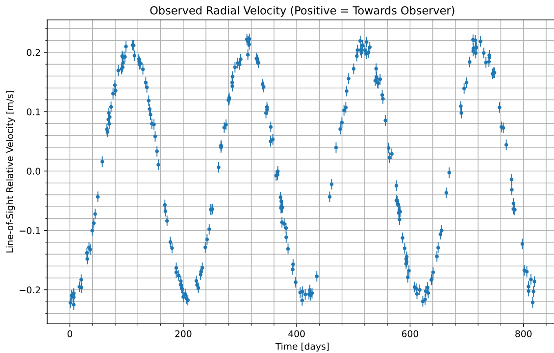
Figure 1: We have isolated the radial velocity of the host star due to the candidate planet. Data begins at UTC 2069-03-25/14:50. Positive values indicate the velocity at which the star is moving towards us; negative indicate the velocity at which it is moving away.
