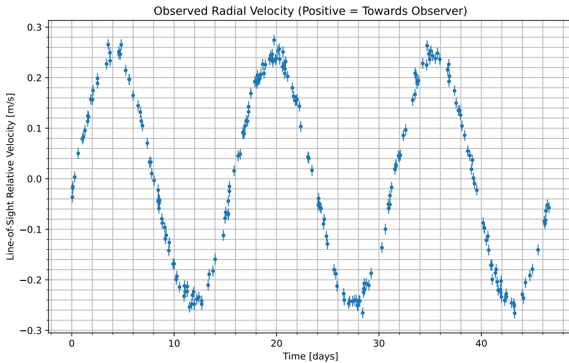
Figure 1: We have isolated the radial velocity of the host star due to the candidate planet. Data begins at UTC 2085-08-26/22:52. Positive values indicate the velocity at which the star is moving towards us; negative indicate the velocity at which it is moving away.
