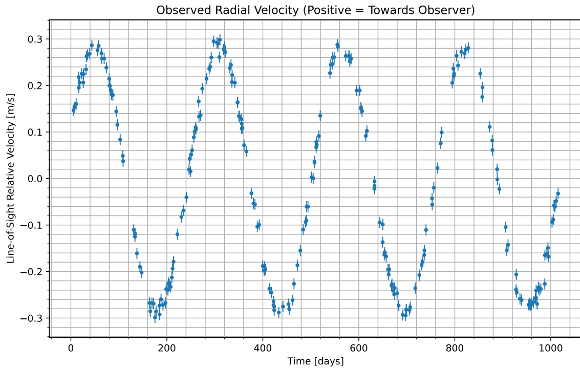
Figure 1: We have isolated the radial velocity of the host star due to the candidate planet. Data begins at UTC 2068-12-19/17:03. Positive values indicate the velocity at which the star is moving towards us; negative indicate the velocity at which it is moving away.
