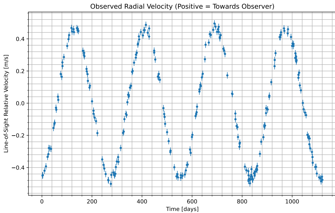
Figure 1: We have isolated the radial velocity of the host star due to the candidate planet. Data begins at UTC 2092-04-04/21:20. Positive values indicate the velocity at which the star is moving towards us; negative indicate the velocity at which it is moving away.
