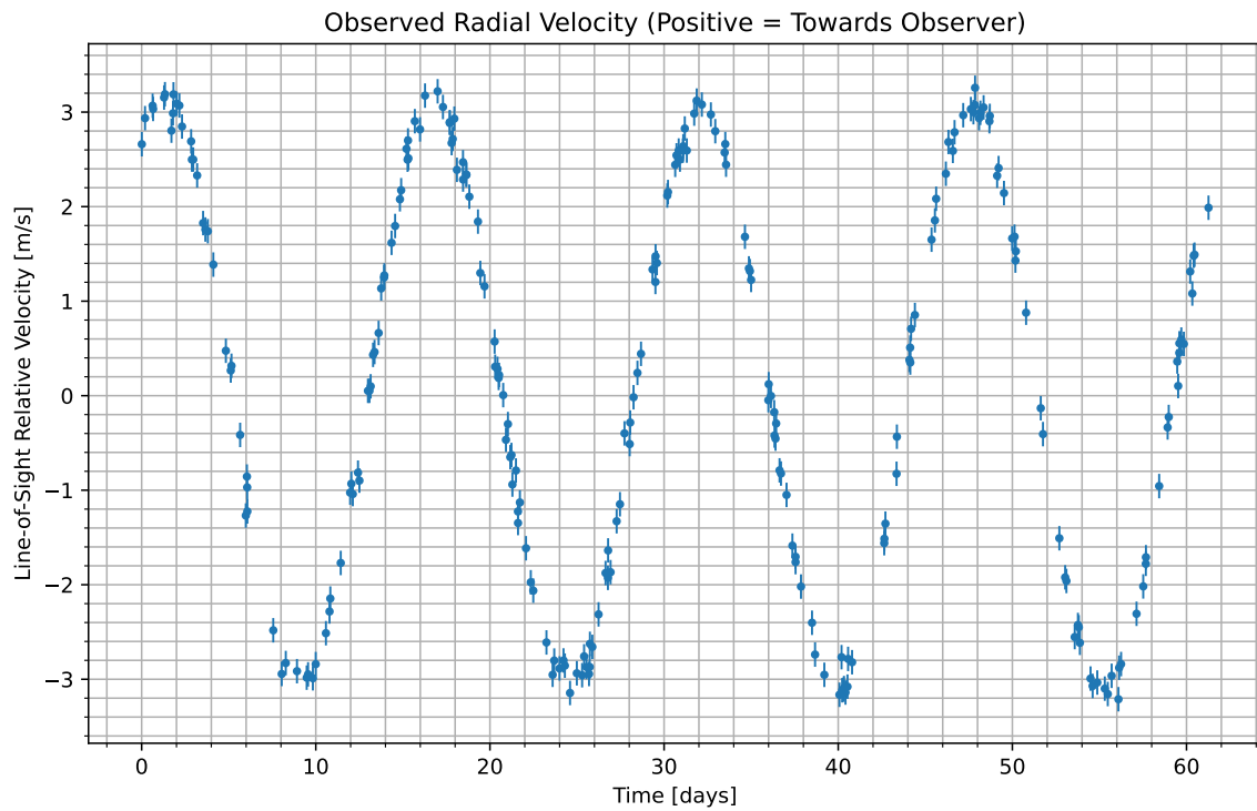
Figure 1: We have isolated the radial velocity of the host star due to the candidate planet. Data begins at UTC 2076-05-18/09:30. Positive values indicate the velocity at which the star is moving towards us; negative indicate the velocity at which it is moving away.
