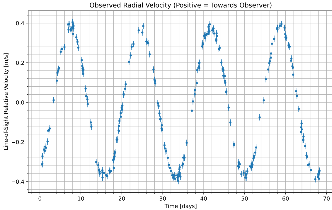
Figure 1: We have isolated the radial velocity of the host star due to the candidate planet. Data begins at UTC 2097-04-05/23:30. Positive values indicate the velocity at which the star is moving towards us; negative indicate the velocity at which it is moving away.
