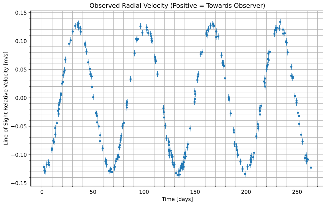
Figure 1: We have isolated the radial velocity of the host star due to the candidate planet. Data begins at UTC 2098-09-20/23:42. Positive values indicate the velocity at which the star is moving towards us; negative indicate the velocity at which it is moving away.
