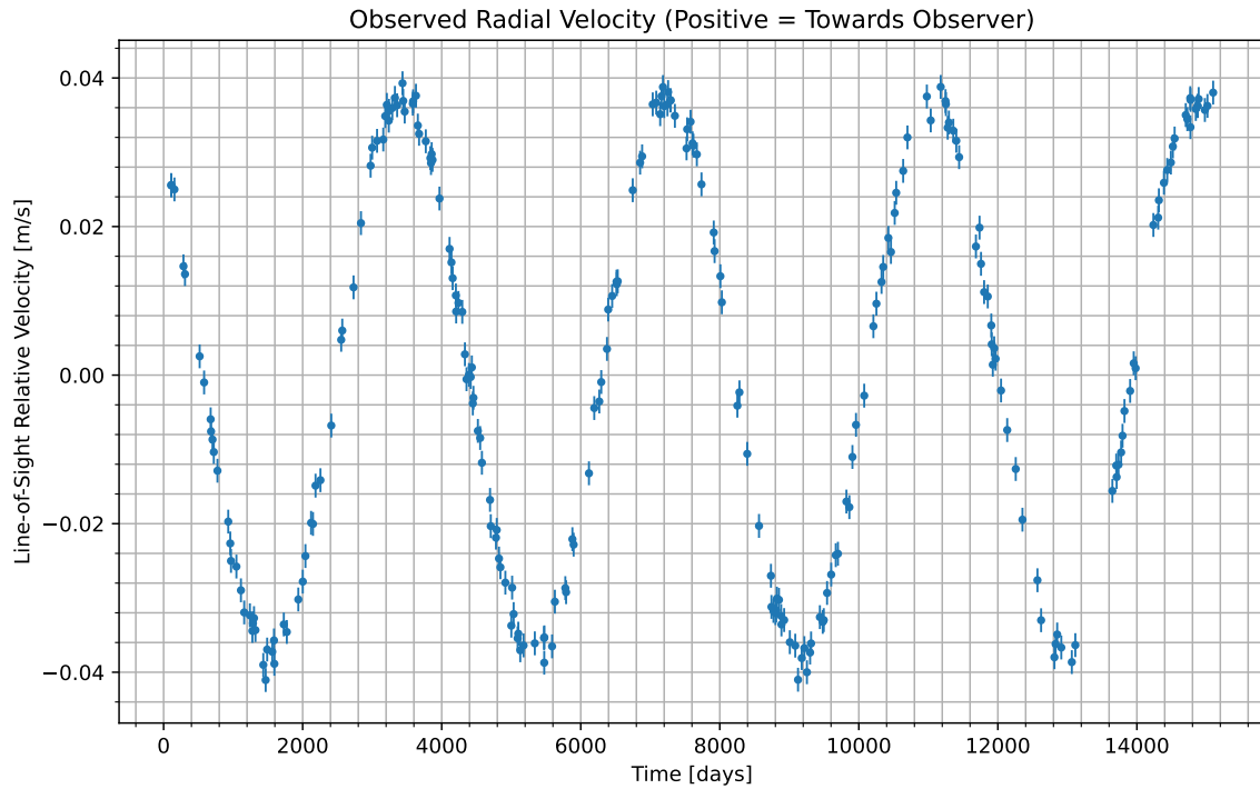
Figure 1: We have isolated the radial velocity of the host star due to the candidate planet. Data begins at UTC 2055-02-07/18:29. Positive values indicate the velocity at which the star is moving towards us; negative indicate the velocity at which it is moving away.
