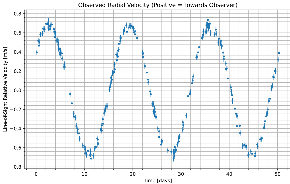
Figure 1: We have isolated the radial velocity of the host star due to the candidate planet. Data begins at UTC 2079-06-08/08:39. Positive values indicate the velocity at which the star is moving towards us; negative indicate the velocity at which it is moving away.
