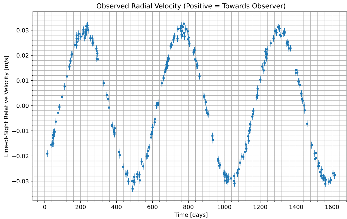
Figure 1: We have isolated the radial velocity of the host star due to the candidate planet. Data begins at UTC 2082-07-25/21:20. Positive values indicate the velocity at which the star is moving towards us; negative indicate the velocity at which it is moving away.
