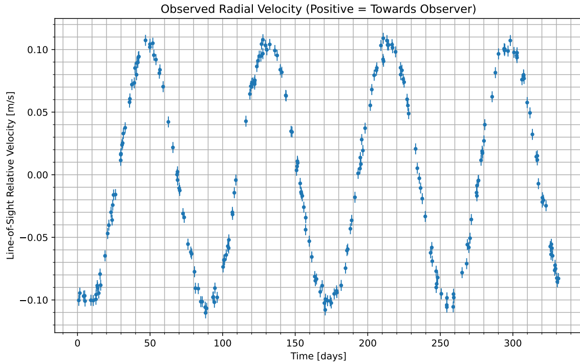
Figure 1: We have isolated the radial velocity of the host star due to the candidate planet. Data begins at UTC 2096-05-30/19:47. Positive values indicate the velocity at which the star is moving towards us; negative indicate the velocity at which it is moving away.
