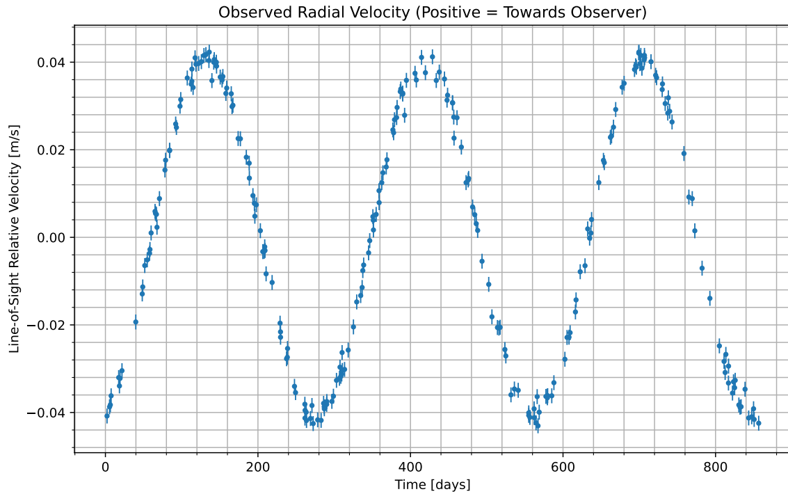
Figure 1: We have isolated the radial velocity of the host star due to the candidate planet. Data begins at UTC 2094-08-18/05:44. Positive values indicate the velocity at which the star is moving towards us; negative indicate the velocity at which it is moving away.
