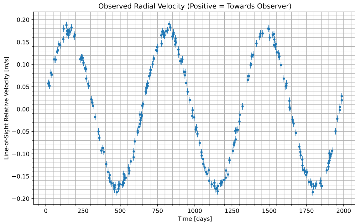
Figure 1: We have isolated the radial velocity of the host star due to the candidate planet. Data begins at UTC 2077-05-21/04:46. Positive values indicate the velocity at which the star is moving towards us; negative indicate the velocity at which it is moving away.
