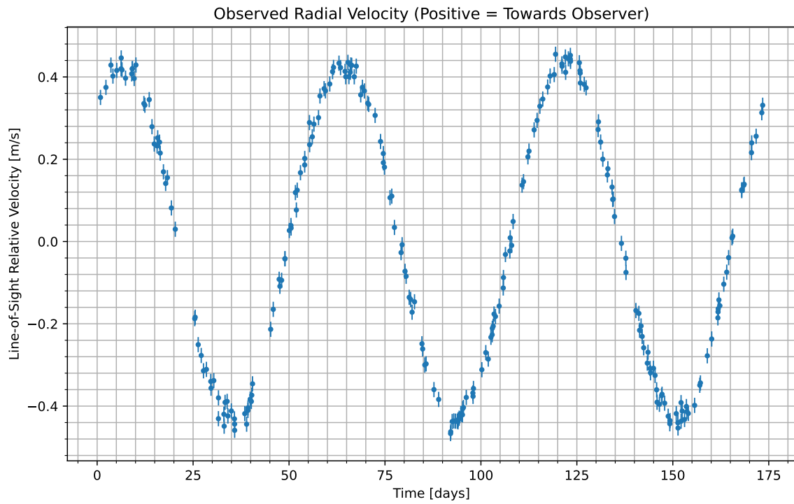
Figure 1: We have isolated the radial velocity of the host star due to the candidate planet. Data begins at UTC 2097-10-19/17:04. Positive values indicate the velocity at which the star is moving towards us; negative indicate the velocity at which it is moving away.
