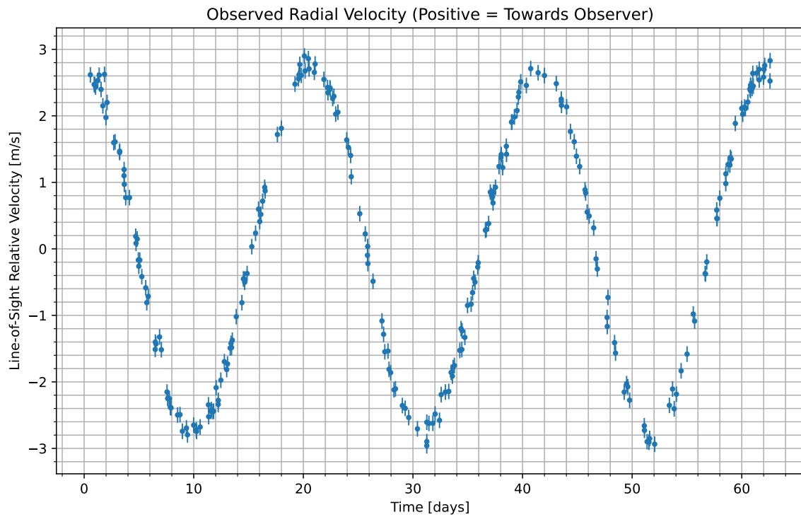
Figure 1: We have isolated the radial velocity of the host star due to the candidate planet. Data begins at UTC 2078-09-09/00:28. Positive values indicate the velocity at which the star is moving towards us; negative indicate the velocity at which it is moving away.
