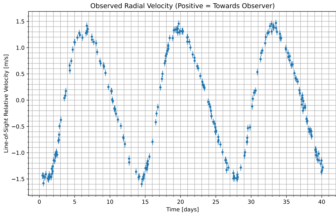
Figure 1: We have isolated the radial velocity of the host star due to the candidate planet. Data begins at UTC 2084-11-05/21:30. Positive values indicate the velocity at which the star is moving towards us; negative indicate the velocity at which it is moving away.
